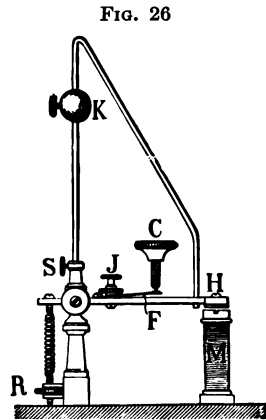
Wagner hammer.
